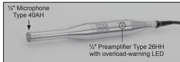
Fig. 1 1/2" Low-noise Level Microphone System Type 40HH
