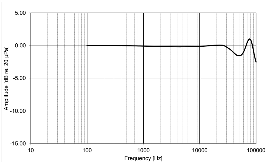
Fig. 2 Typical pressure frequency response for 40LS
