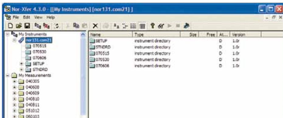
NorXfer screenshot
