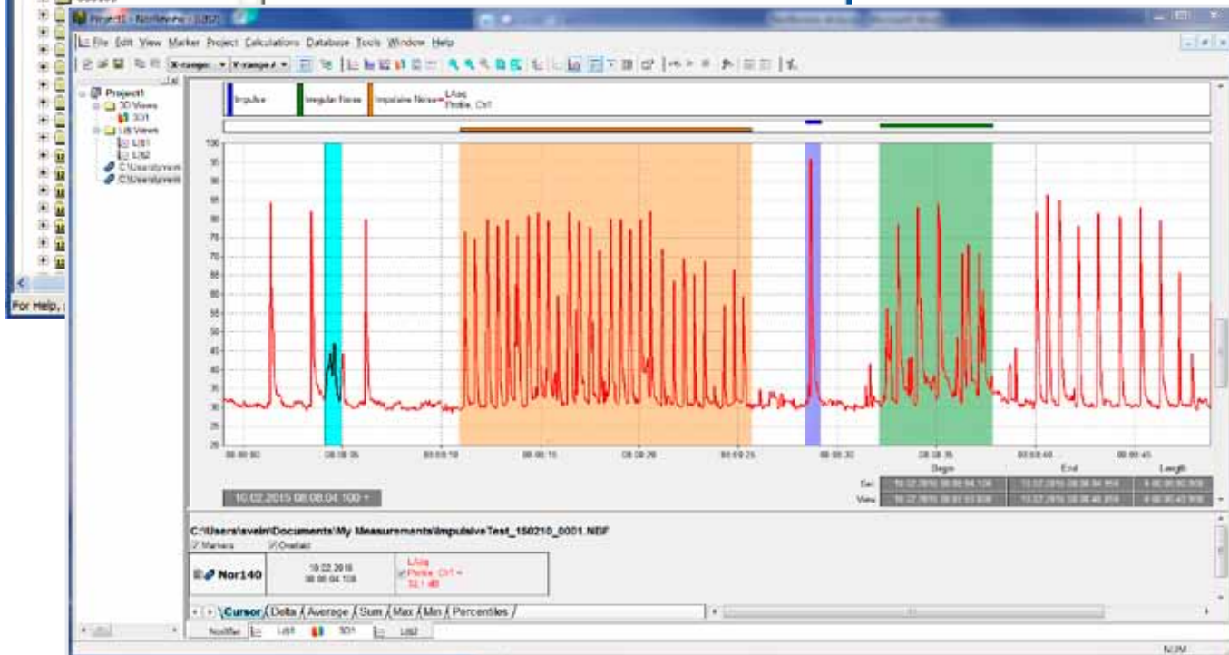
NorReview screenshot
